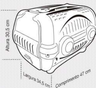
Cod. 01544 Transport Box Luxo N2 Black w/ Gray Furacão Pet
